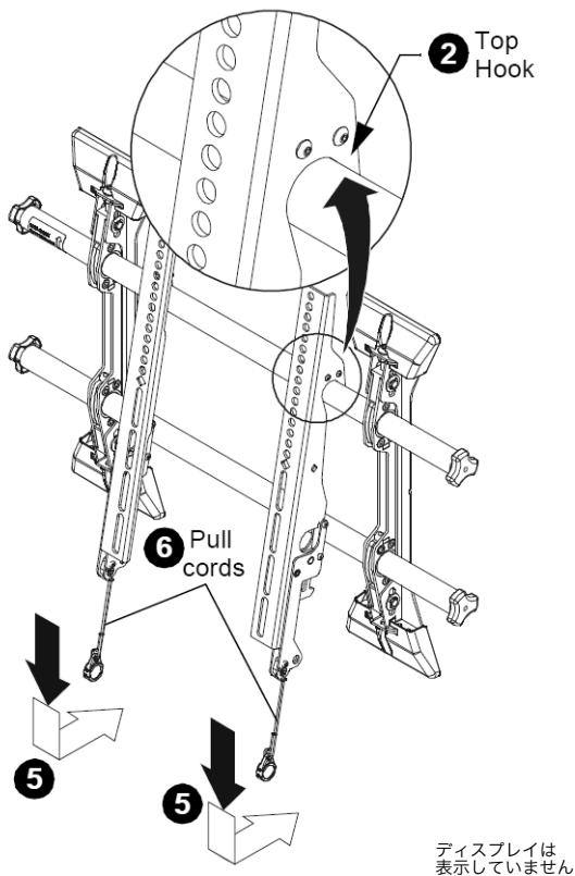
MSM1U / LSM1U
