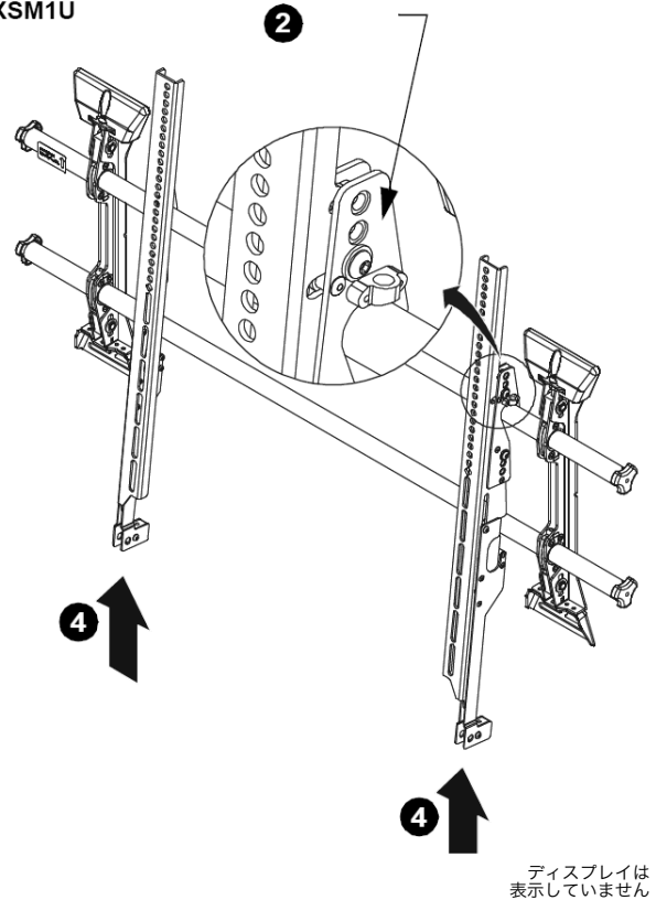
XSM1U
